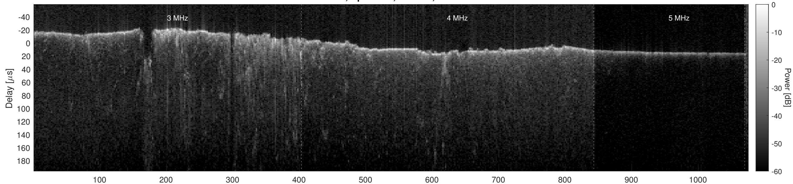
Orbit 6043, Optimized, Window, Channel 2
