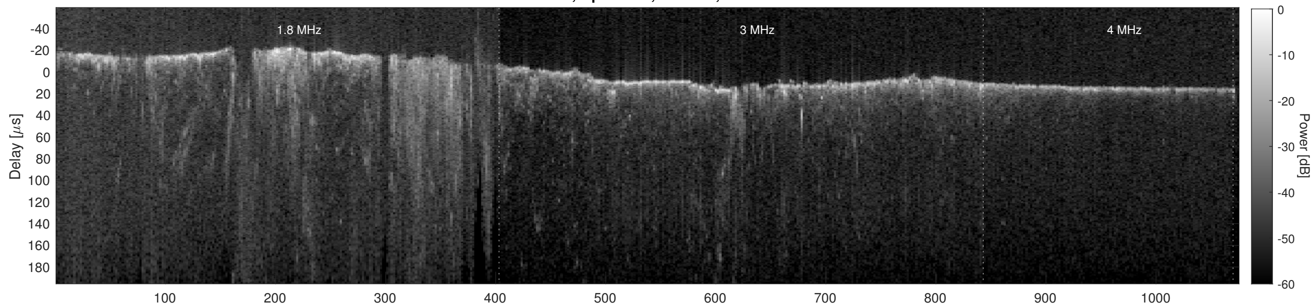
Orbit 6043, Cluttergram
