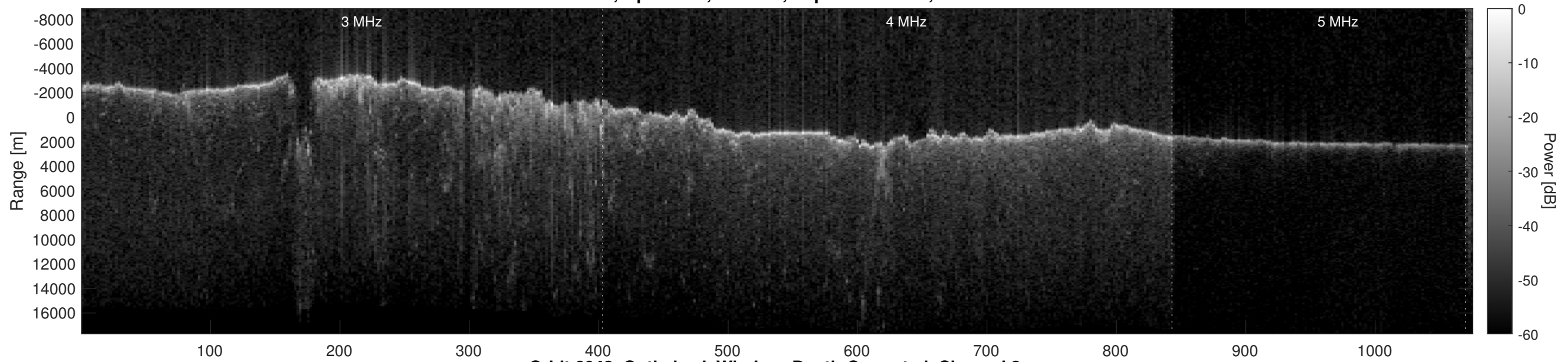
Orbit 6043, Optimized, Window, Depth-Corrected, Channel 2
