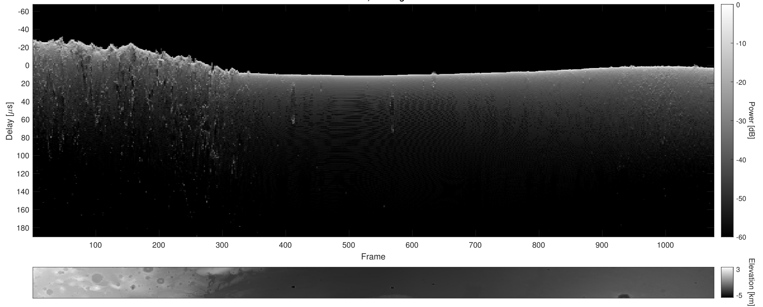
Orbit 6044, Cluttergram
