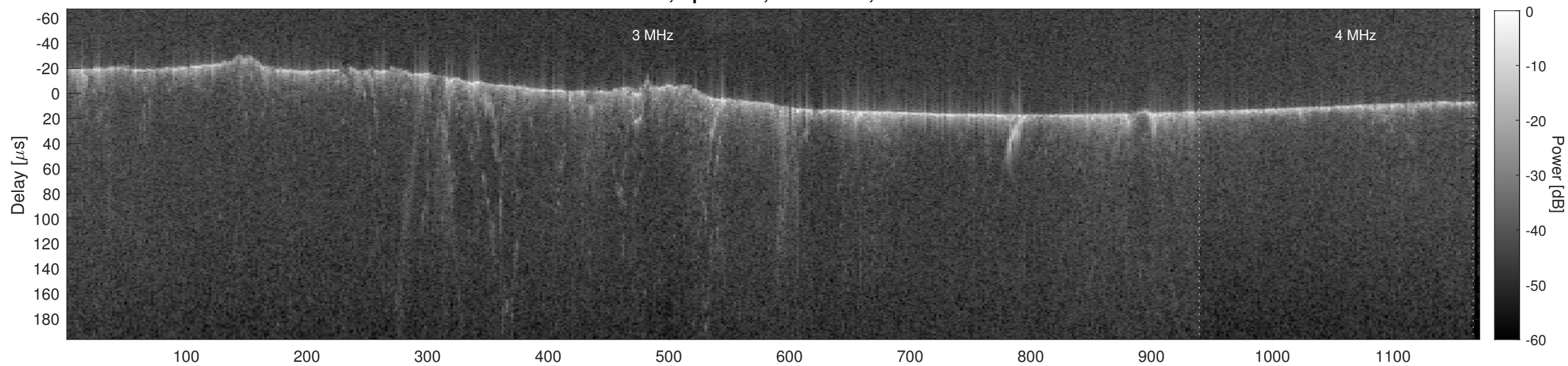
Orbit 6045, Cluttergram
