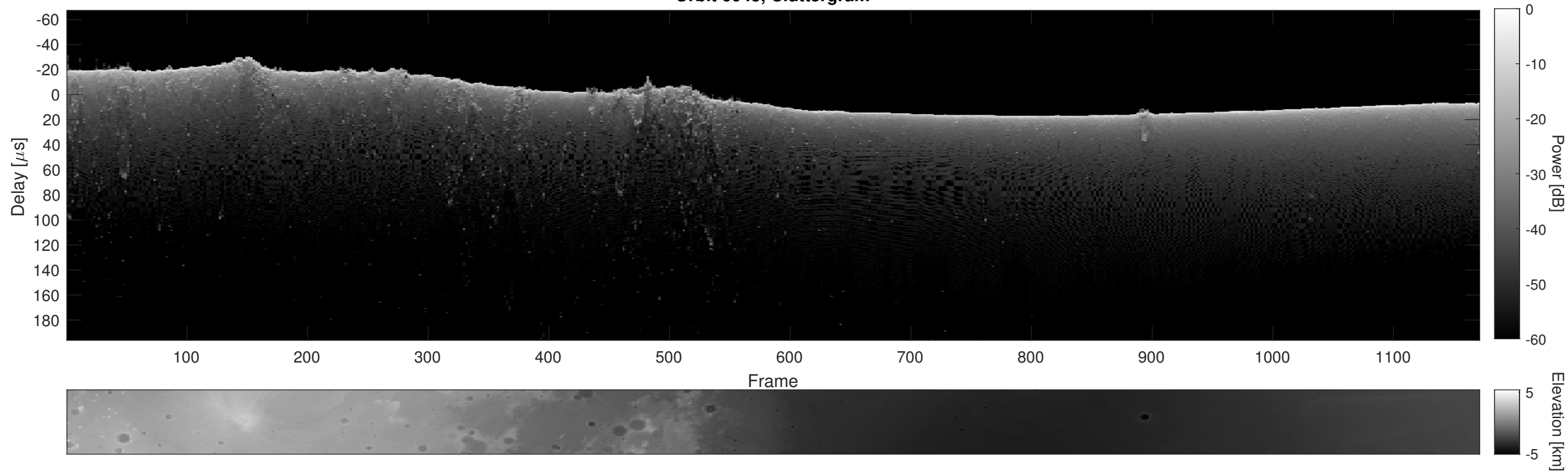
Orbit 6045, Cluttergram
