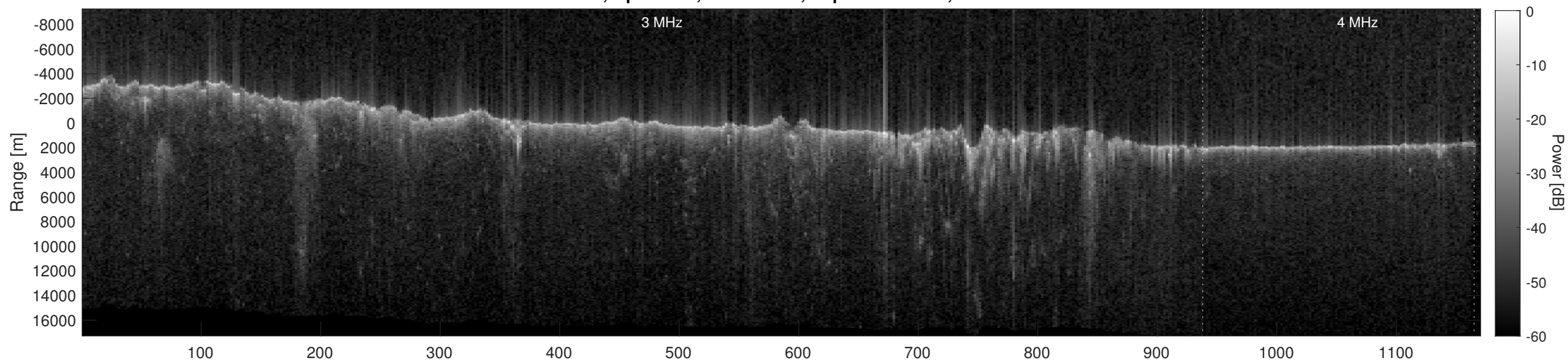
Orbit 6046, Depth-Corrected Cluttergram
