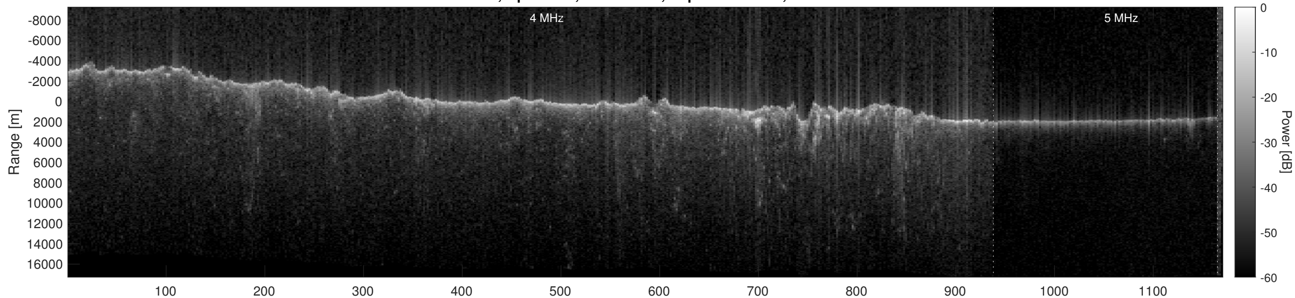
Orbit 6046, Optimized, No Window, Depth-Corrected, Channel 2
