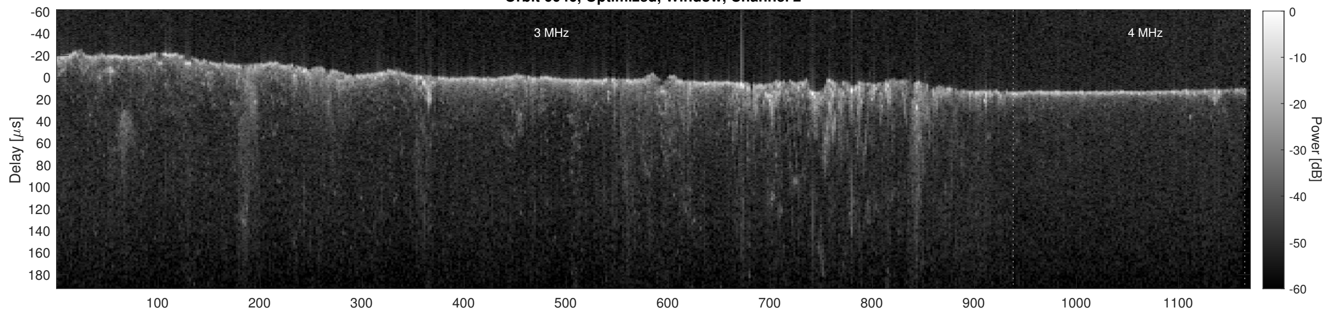
Orbit 6046, Cluttergram
