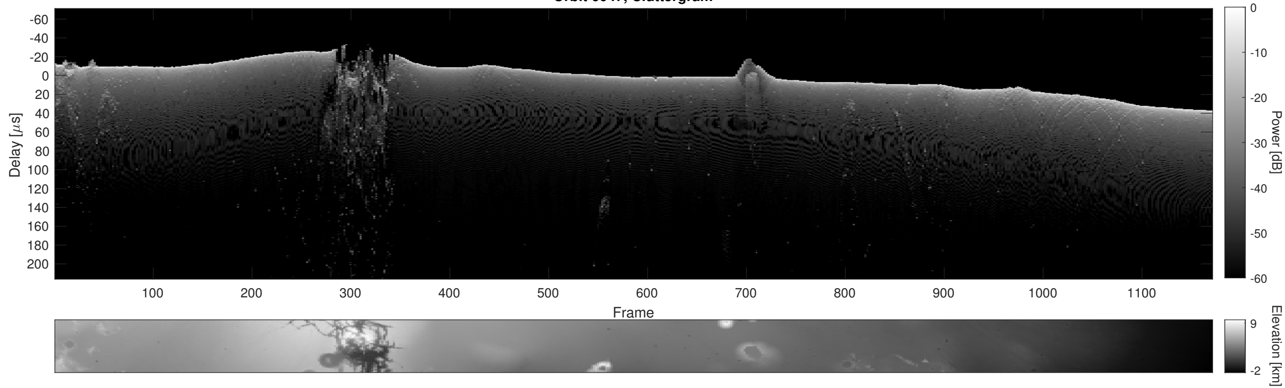
Orbit 6047, Cluttergram
