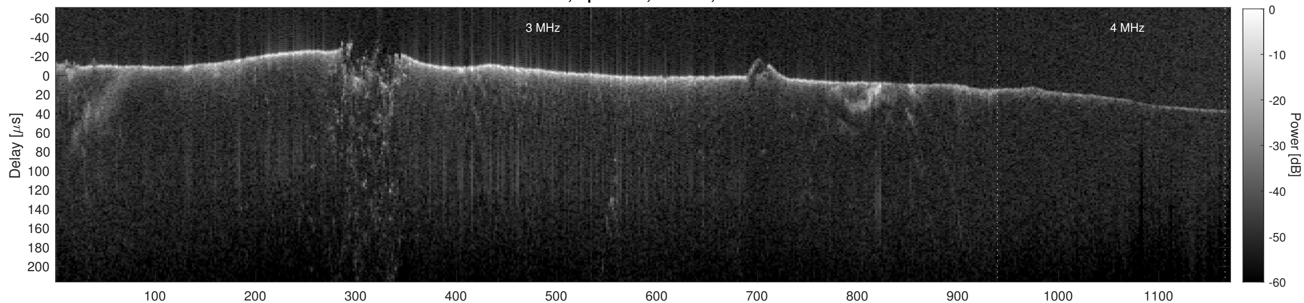
Orbit 6047, Cluttergram
