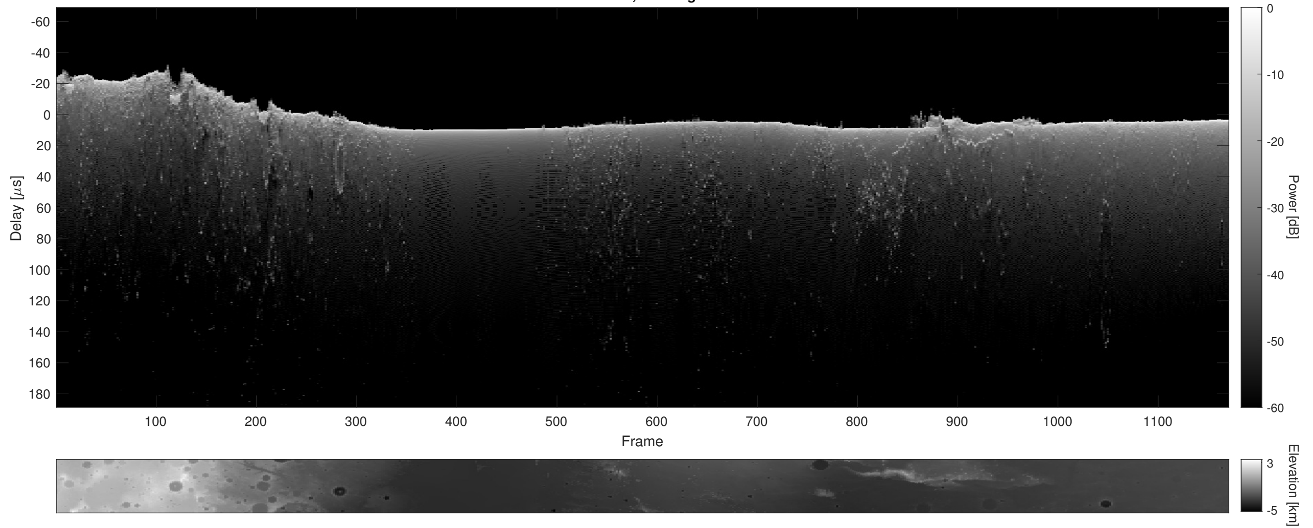
Orbit 6048, Cluttergram
