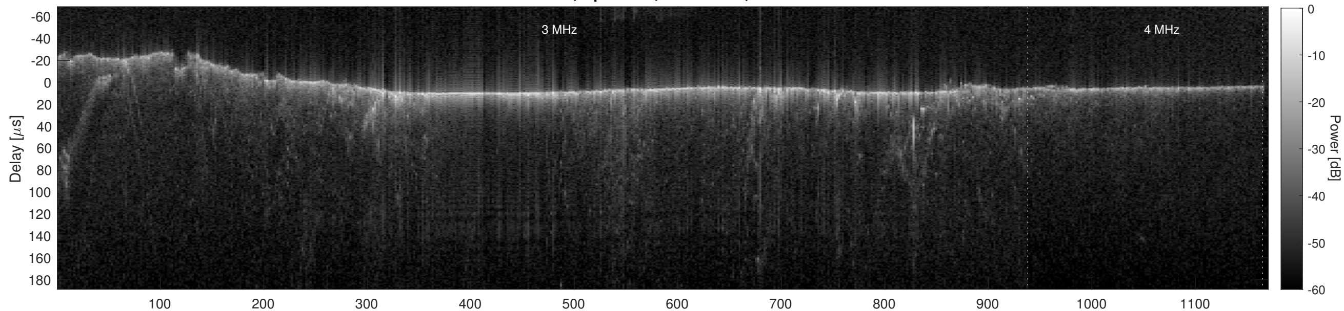
Orbit 6048, Cluttergram
