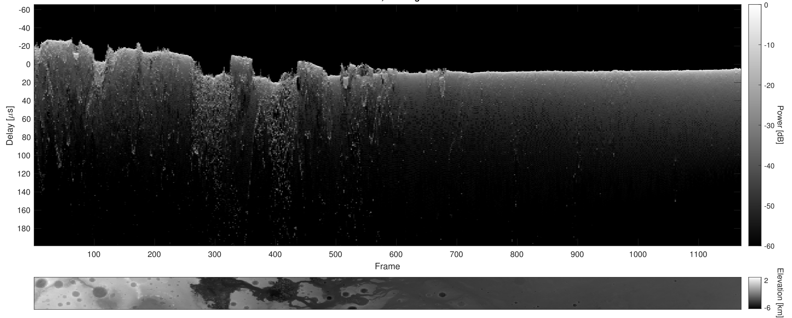
Orbit 6050, Cluttergram
