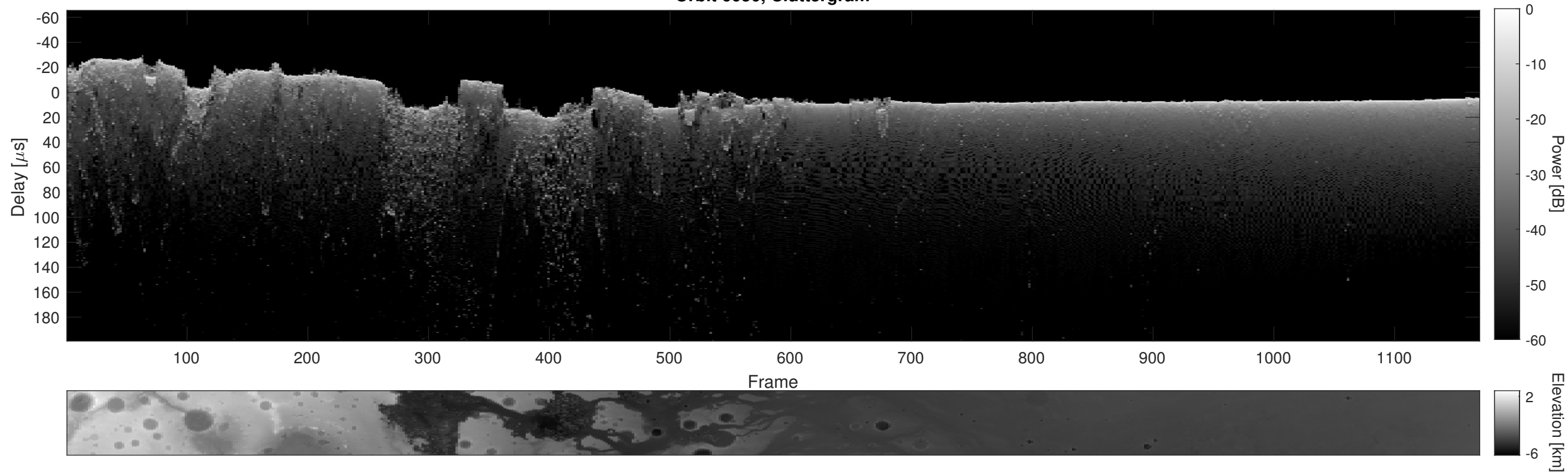
Orbit 6050, Cluttergram
