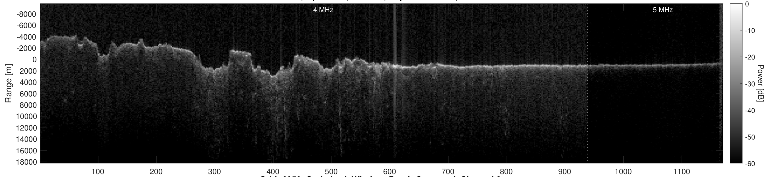
Orbit 6050, Optimized, Window, Depth-Corrected, Channel 2
