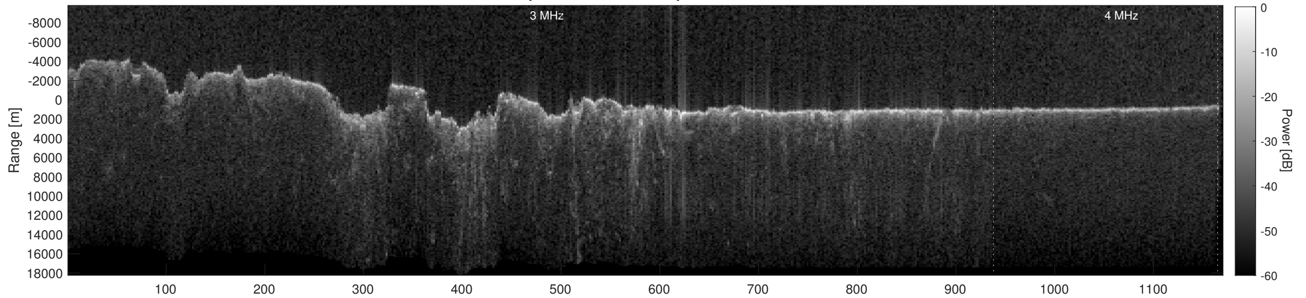
Orbit 6050, Depth-Corrected Cluttergram
