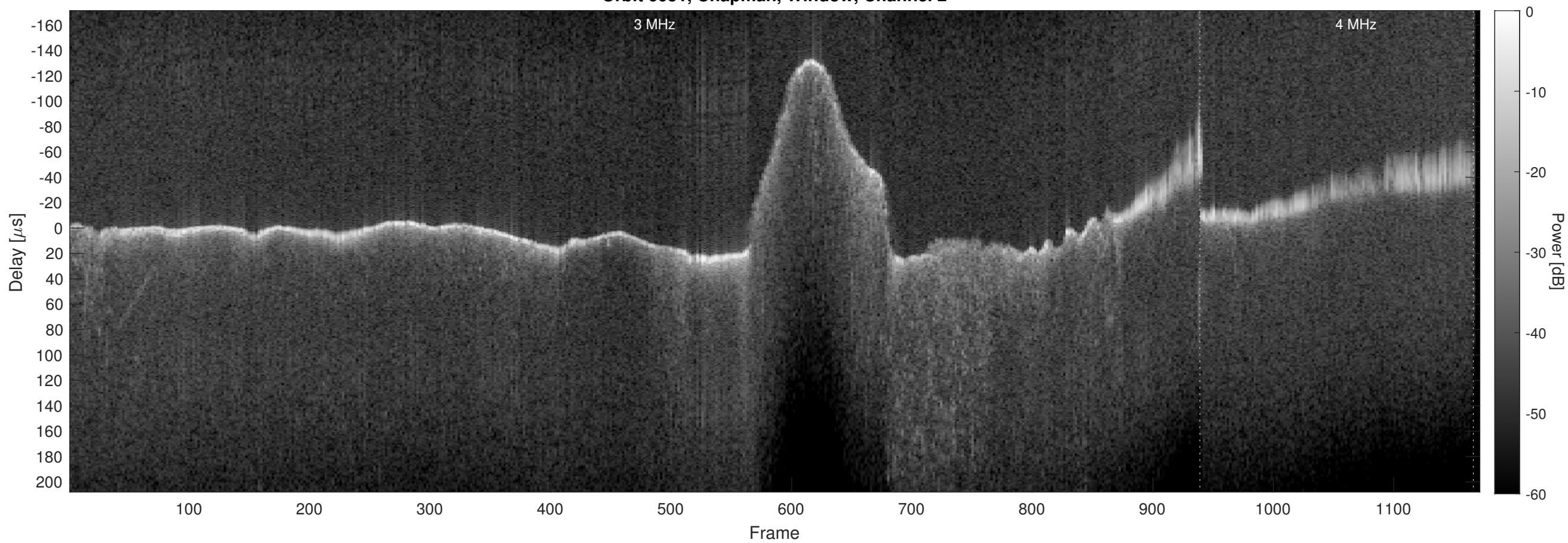
Orbit 6051, Chapman, Window, Channel 2
