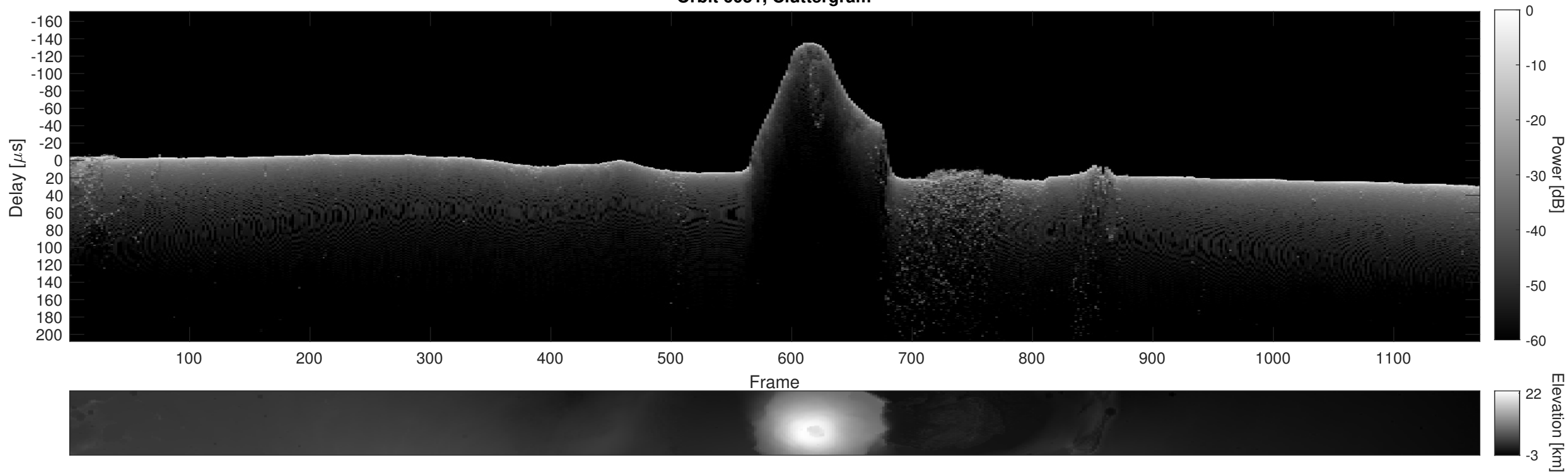
Orbit 6051, Cluttergram
