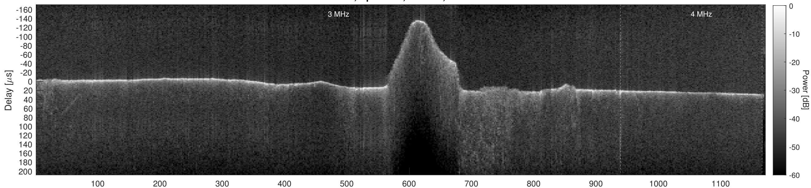
Orbit 6051, Cluttergram
