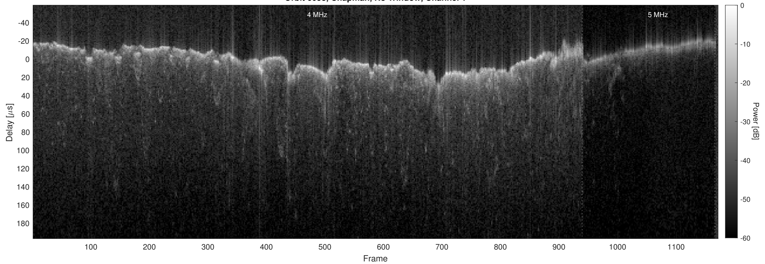
Orbit 6053, Chapman, No Window, Channel 2
