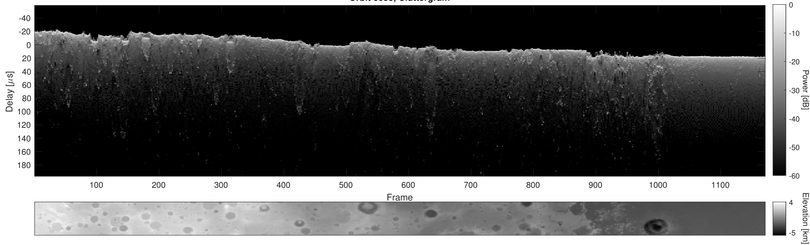
Orbit 6053, Cluttergram
