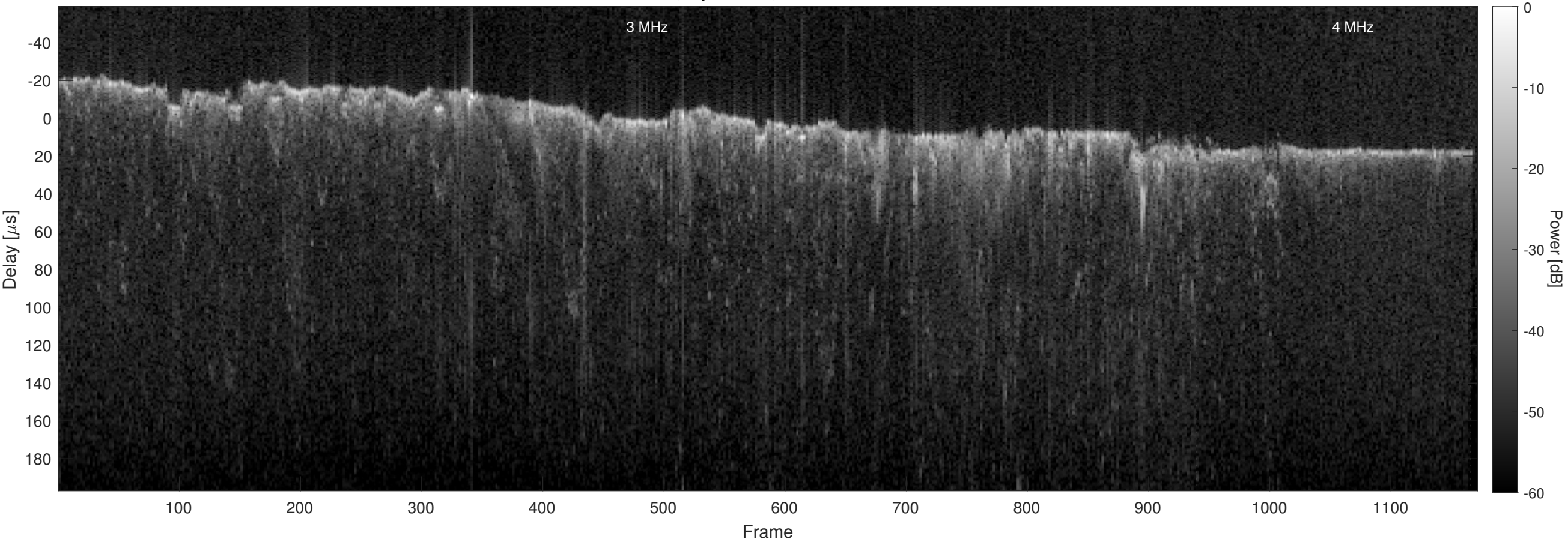
Orbit 6053, Optimized, Window, Channel 2
