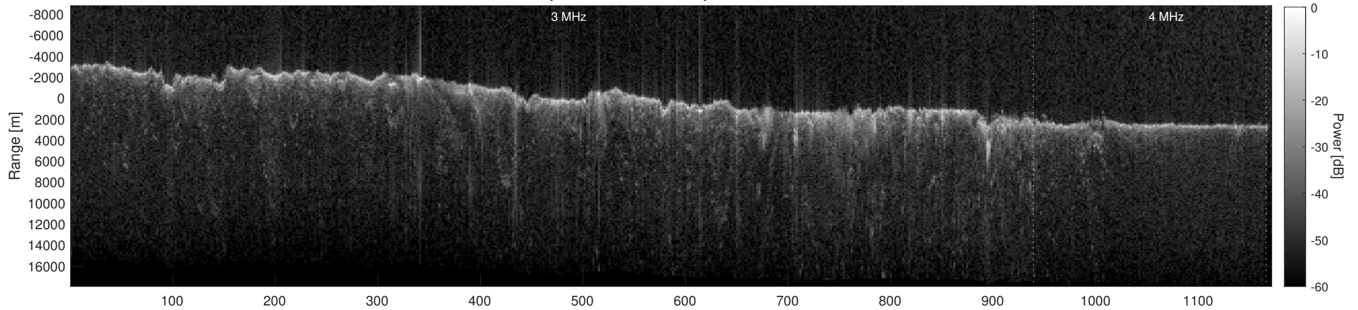
Orbit 6053, Depth-Corrected Cluttergram
