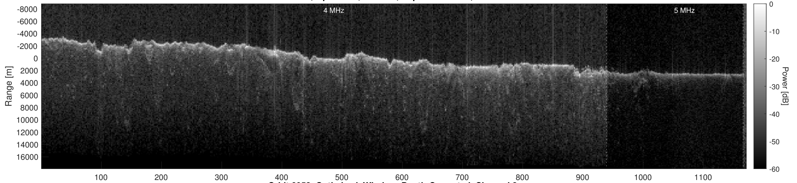
Orbit 6053, Optimized, Window, Depth-Corrected, Channel 2
