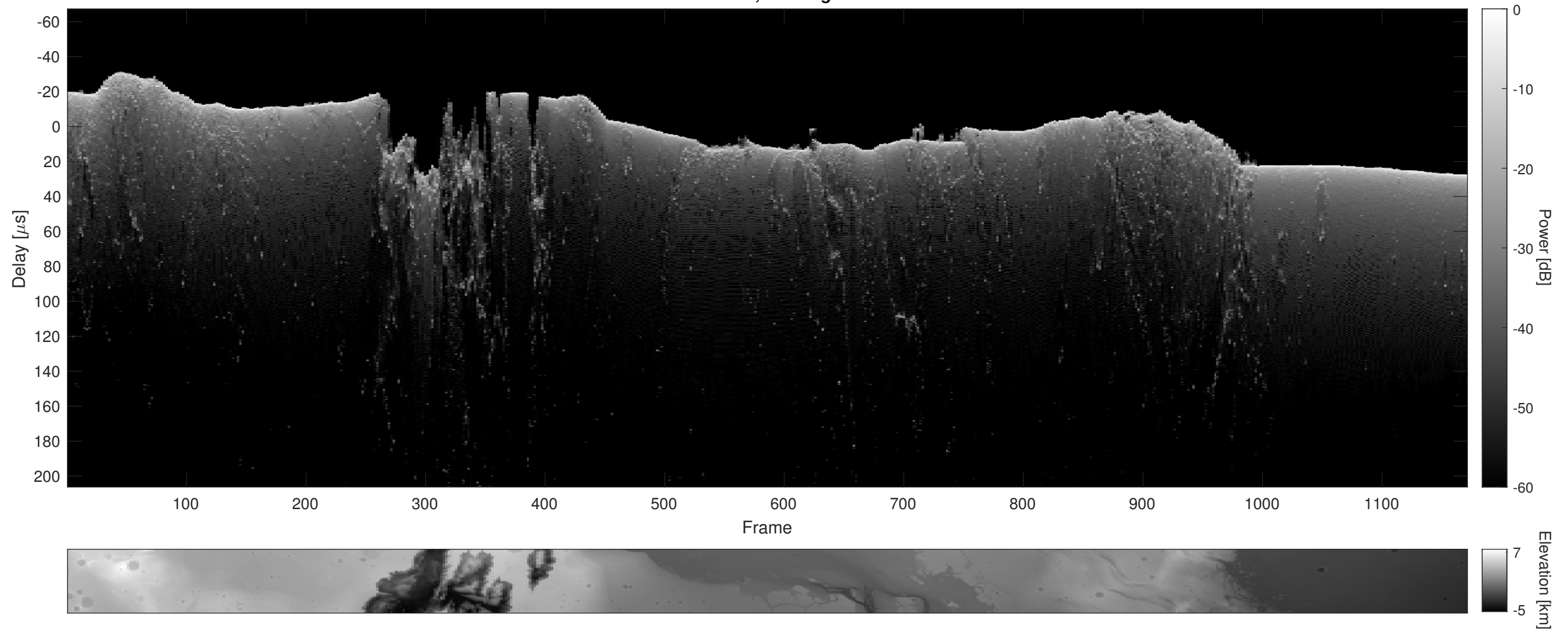
Orbit 6054, Cluttergram
