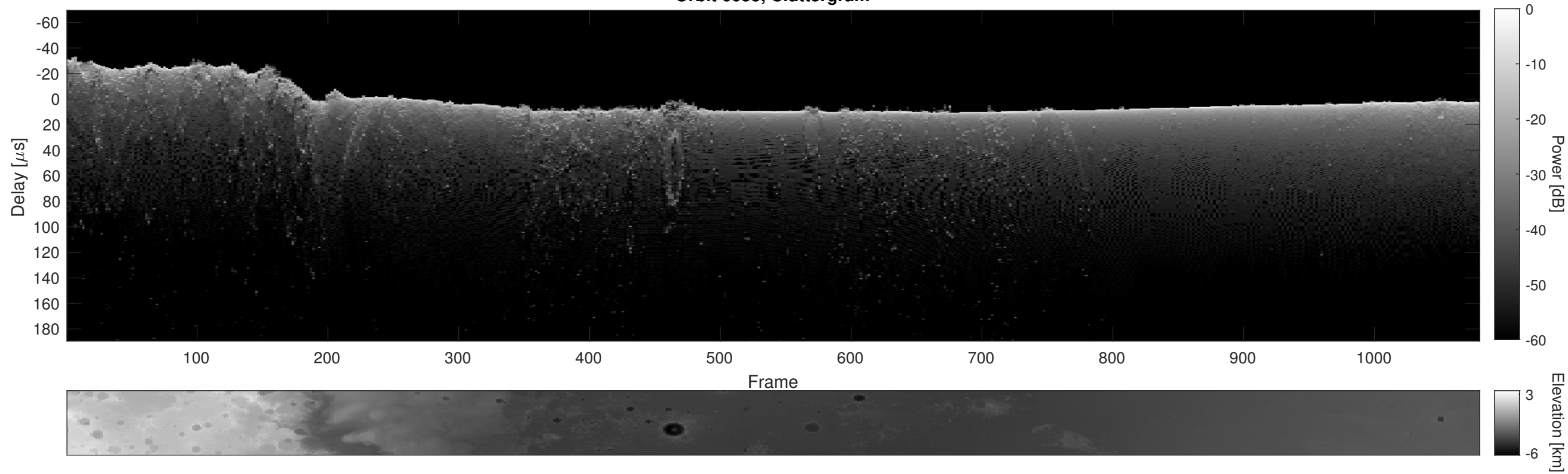
Orbit 6055, Cluttergram
