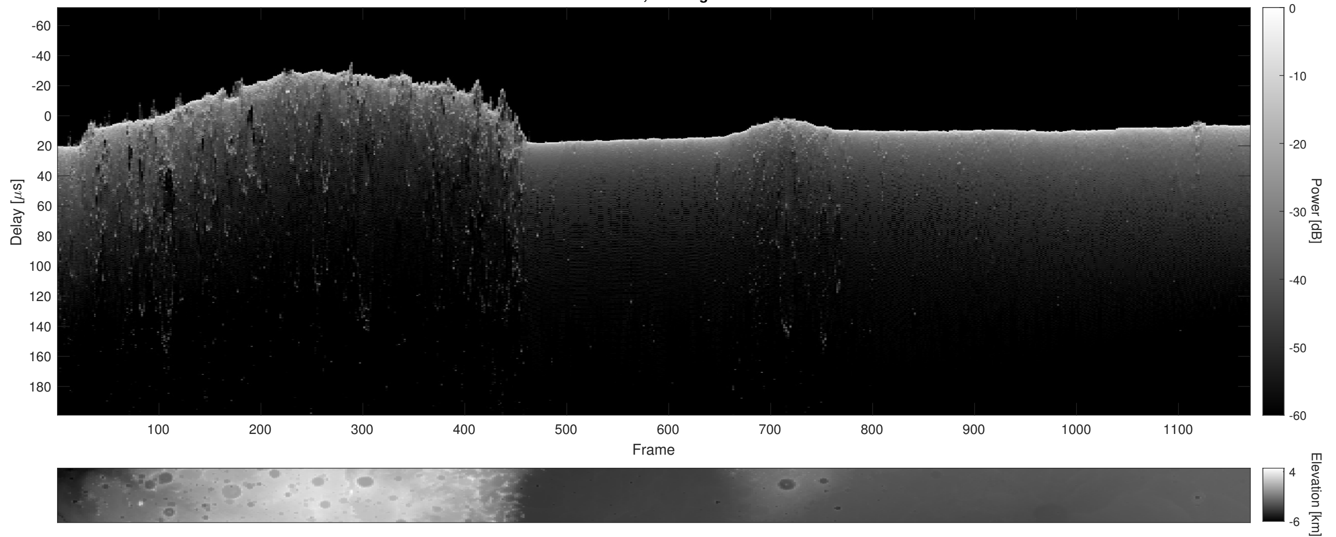
Orbit 6056, Cluttergram
