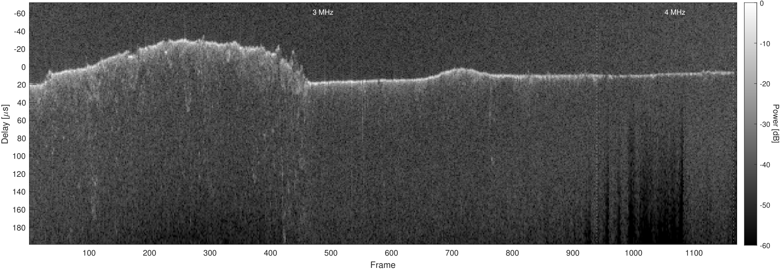
Orbit 6056, Optimized, Window, Channel 2
