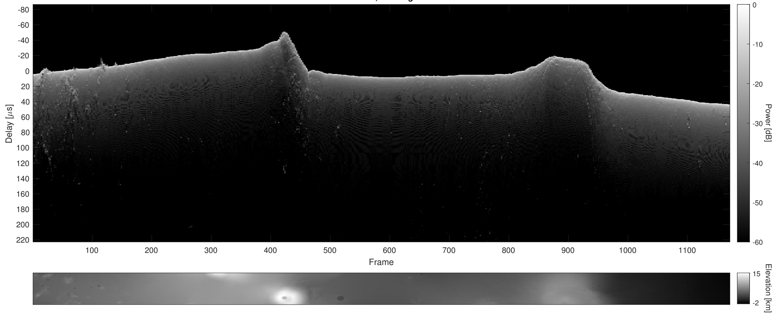
Orbit 6058, Cluttergram
