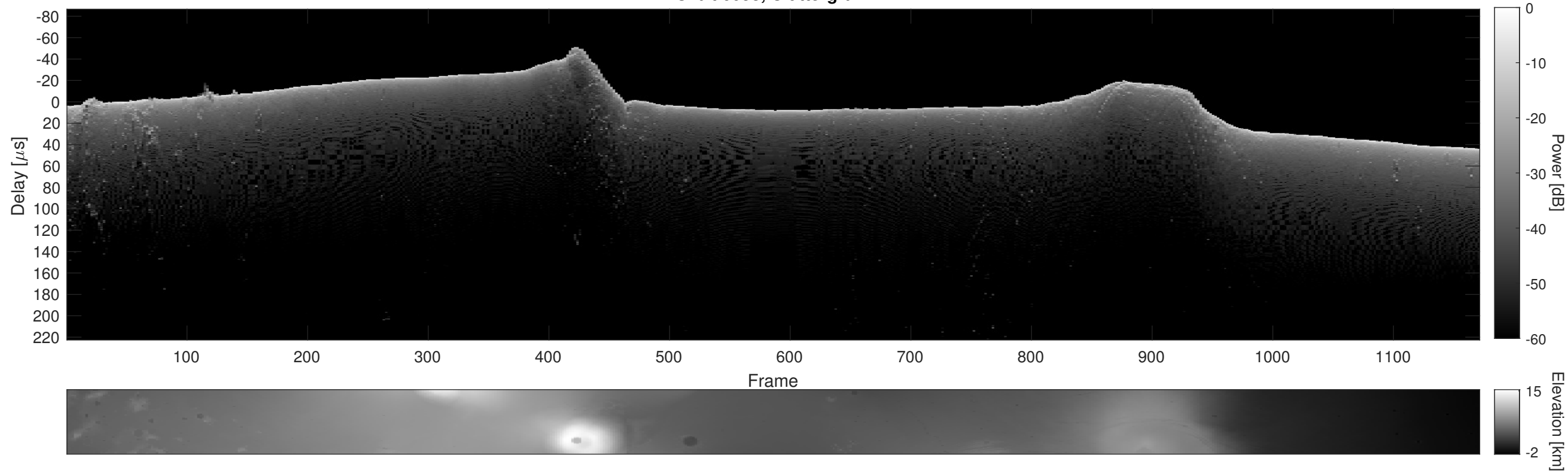
Orbit 6058, Cluttergram
