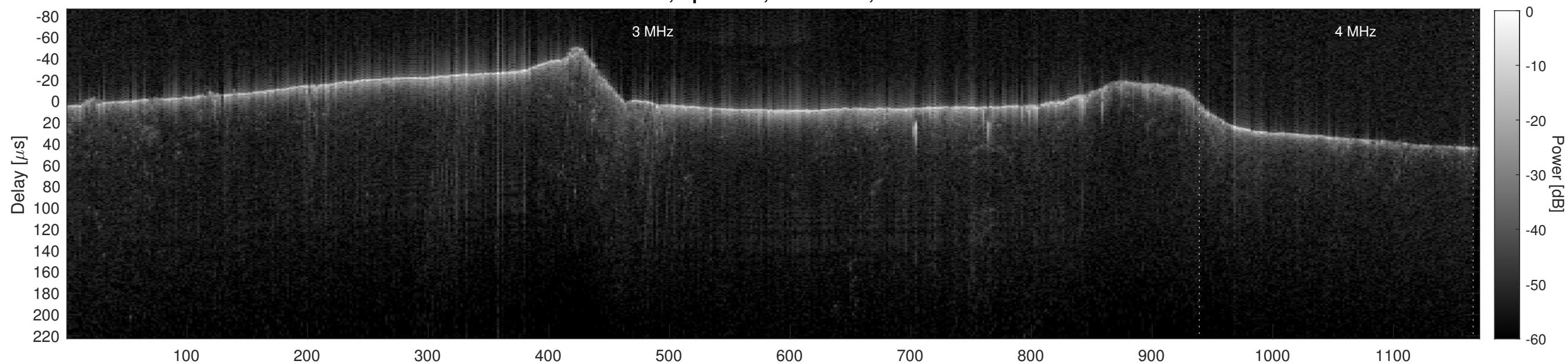
Orbit 6058, Cluttergram
