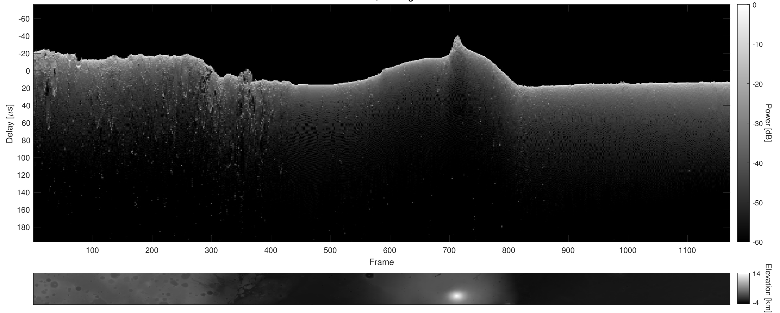
Orbit 6059, Cluttergram
