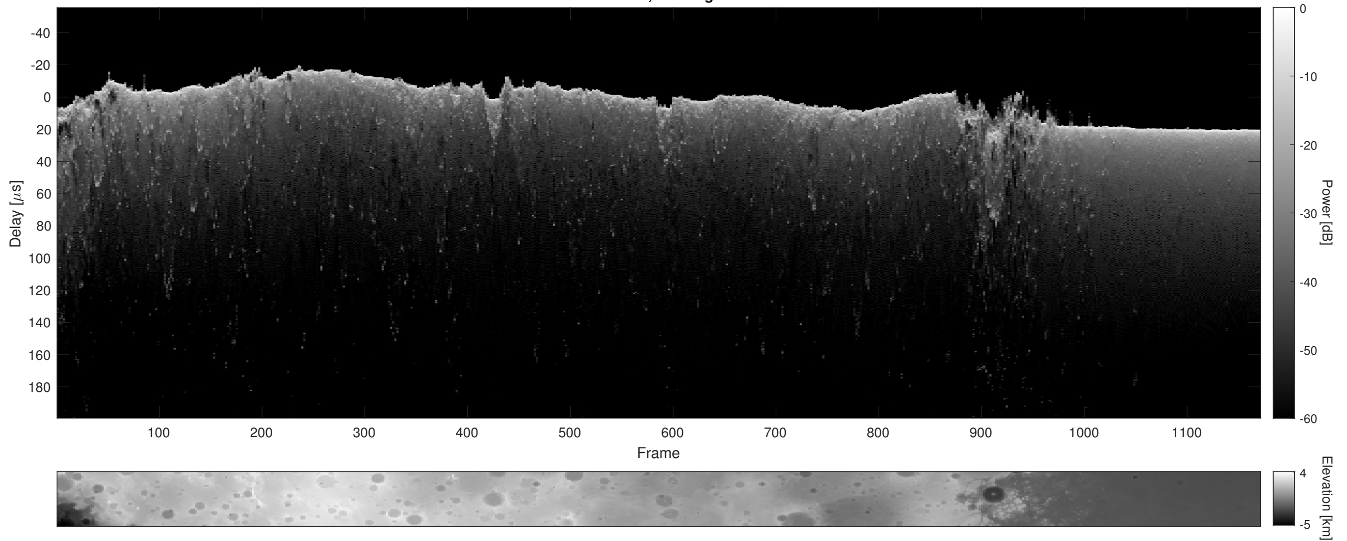
Orbit 6060, Cluttergram
