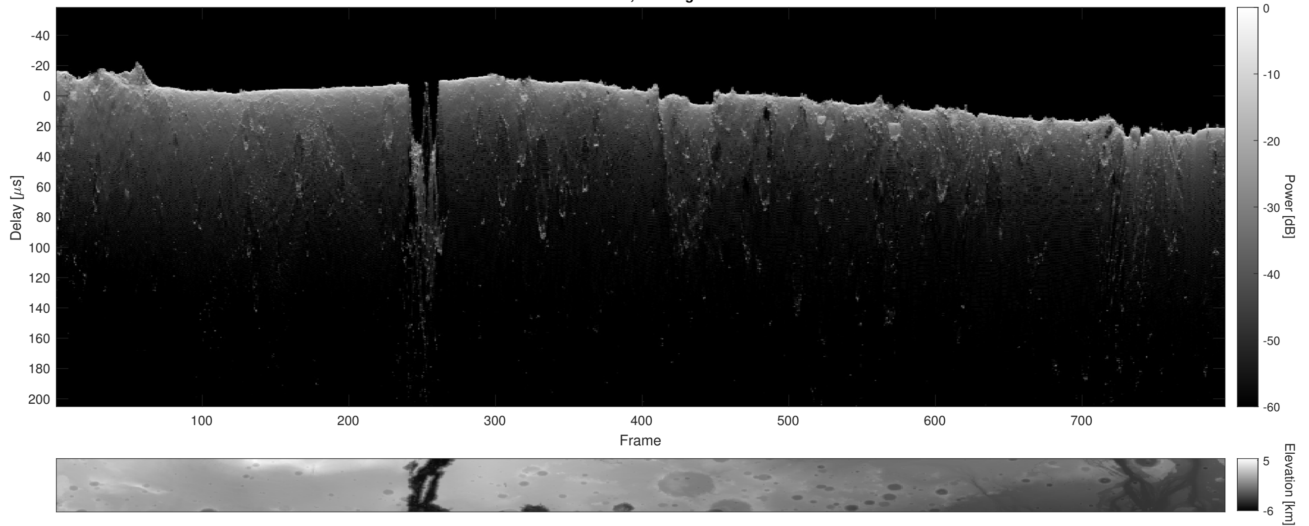
Orbit 6061, Cluttergram
