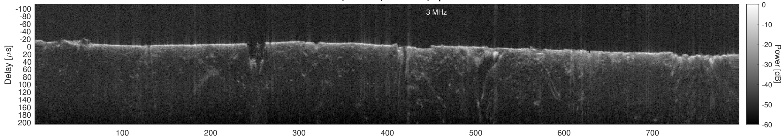
Orbit 6061, Cluttergram
