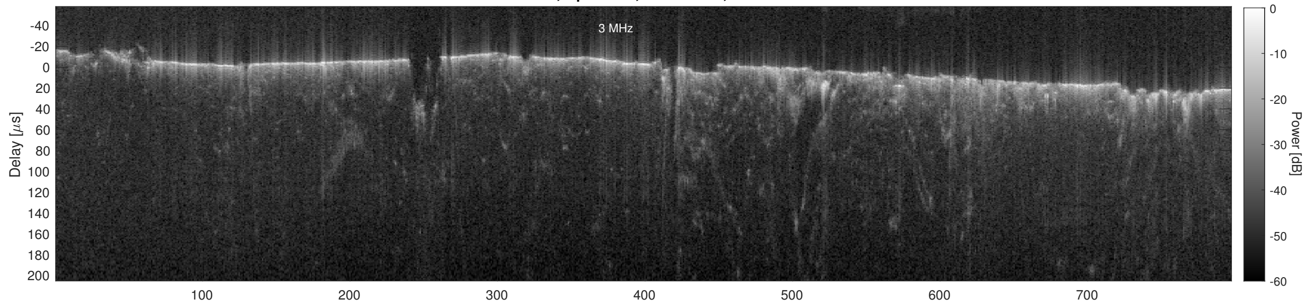
Orbit 6061, Cluttergram
