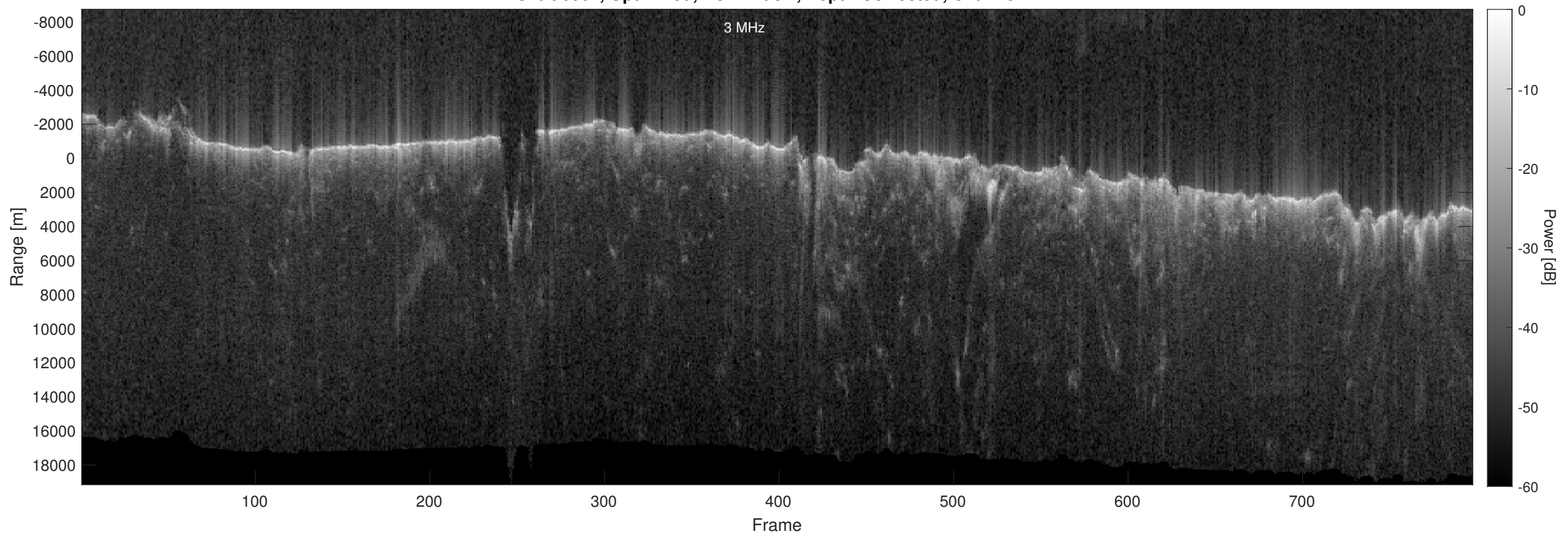
Orbit 6061, Optimized, No Window, Depth-Corrected, Channel 2
