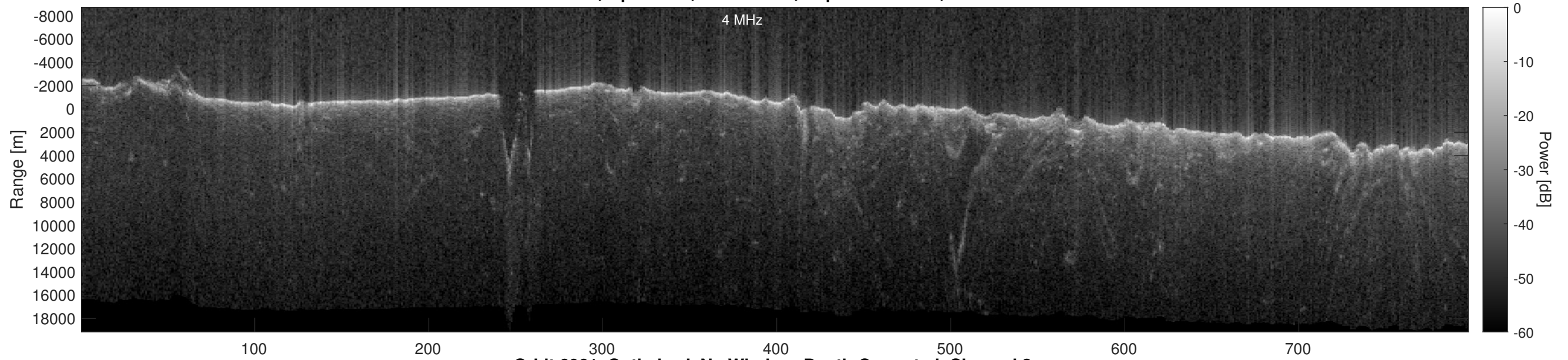
Orbit 6061, Optimized, No Window, Depth-Corrected, Channel 2
