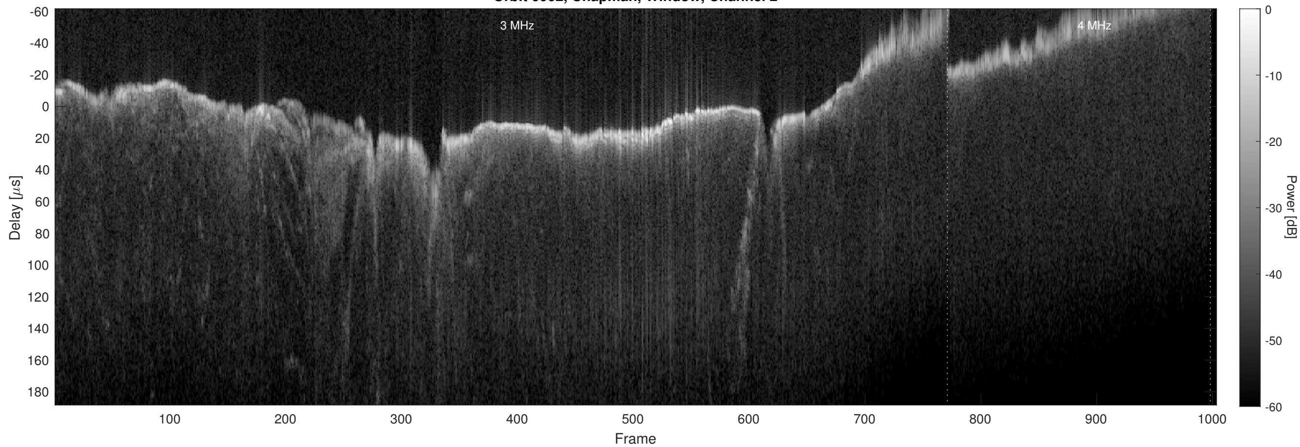
Orbit 6062, Chapman, Window, Channel 2
