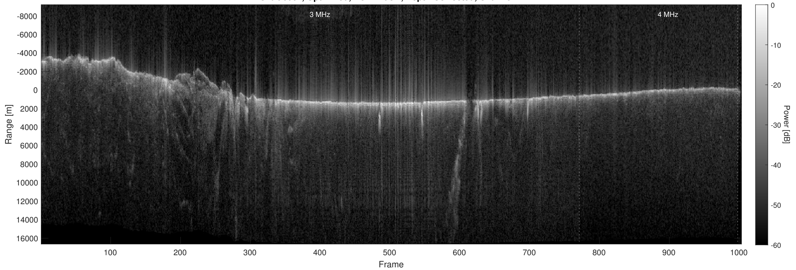
Orbit 6062, Optimized, No Window, Depth-Corrected, Channel 2
