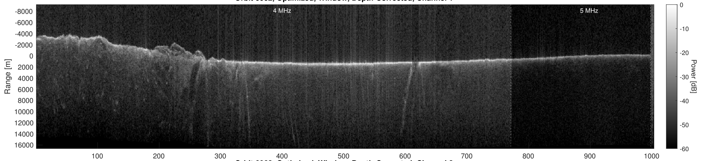
Orbit 6062, Optimized, Window, Depth-Corrected, Channel 2
