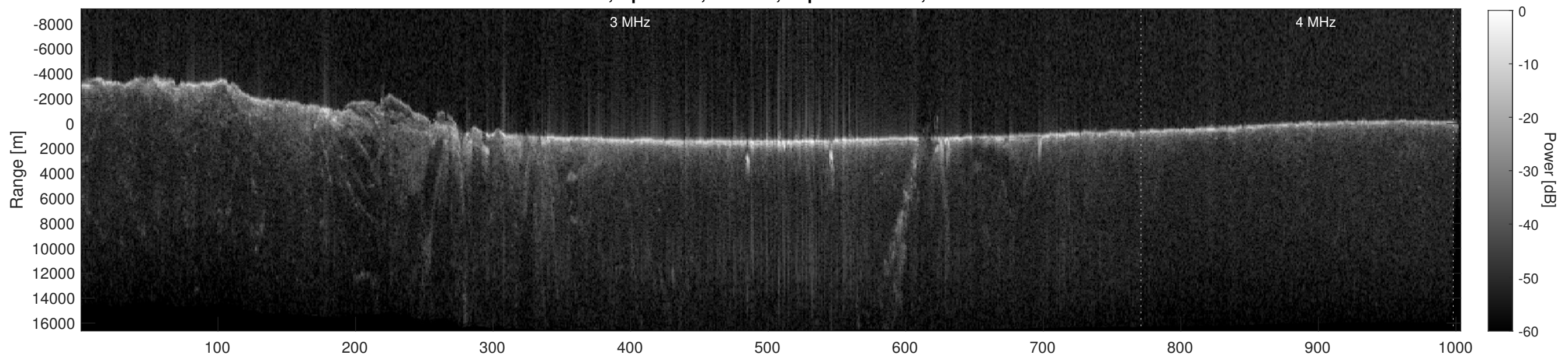
Orbit 6062, Depth-Corrected Cluttergram
