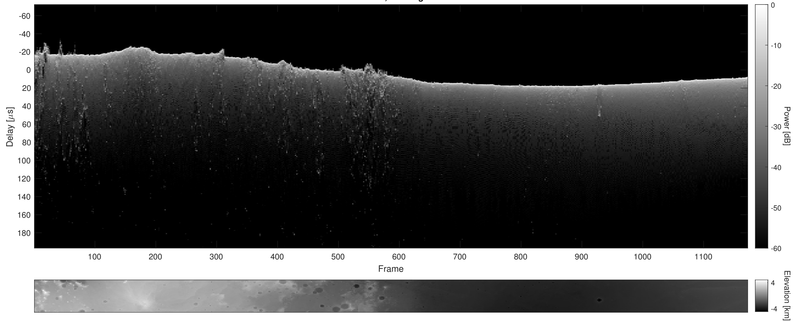
Orbit 6063, Cluttergram
