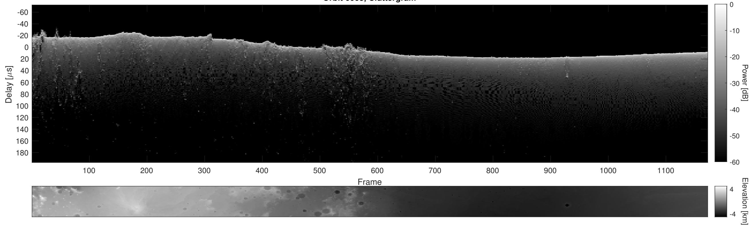
Orbit 6063, Cluttergram
