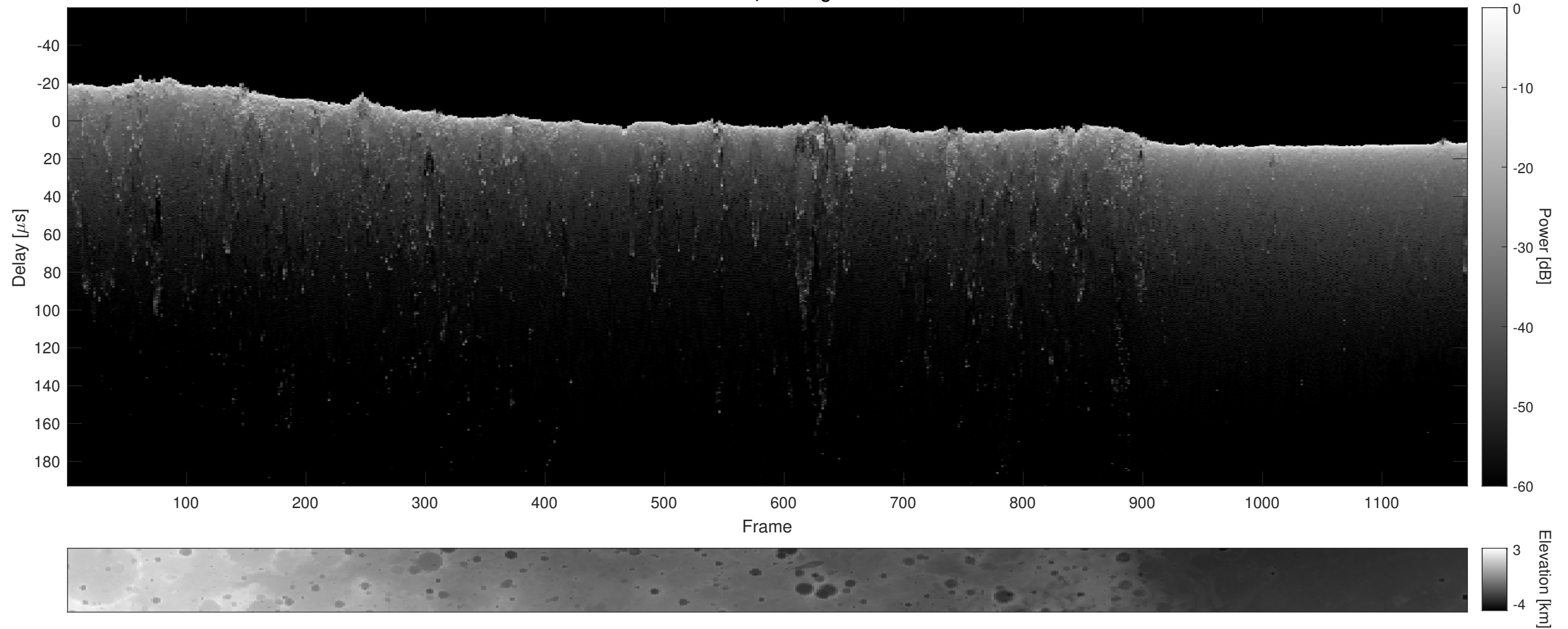
Orbit 6064, Cluttergram
