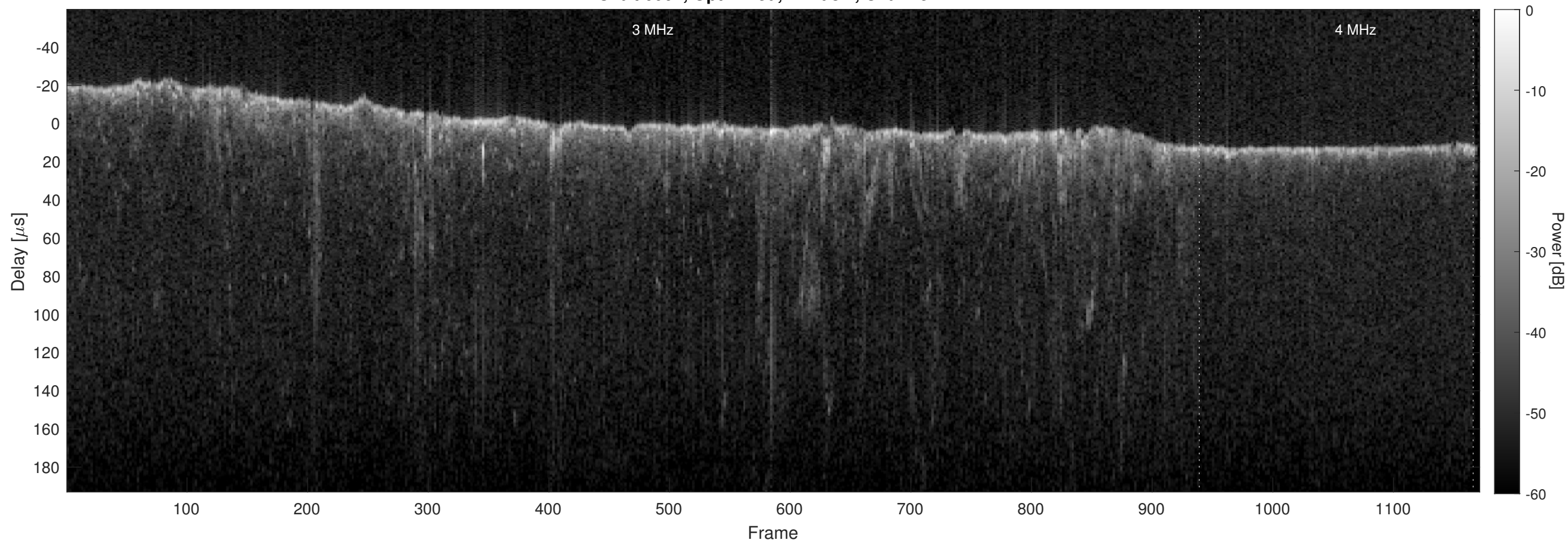
Orbit 6064, Optimized, Window, Channel 2
