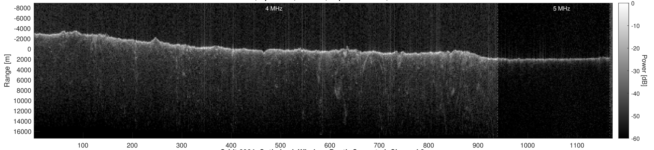
Orbit 6064, Optimized, Window, Depth-Corrected, Channel 2
