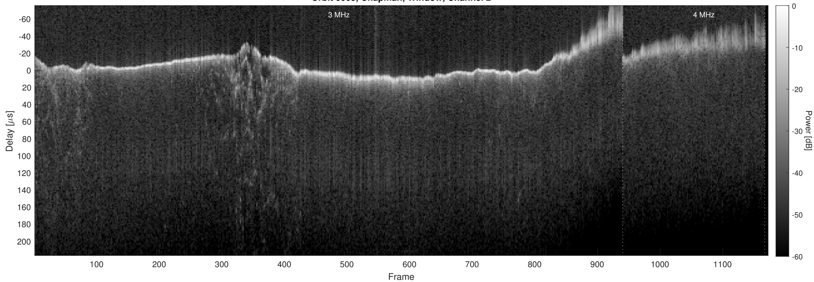
Orbit 6065, Chapman, Window, Channel 2
