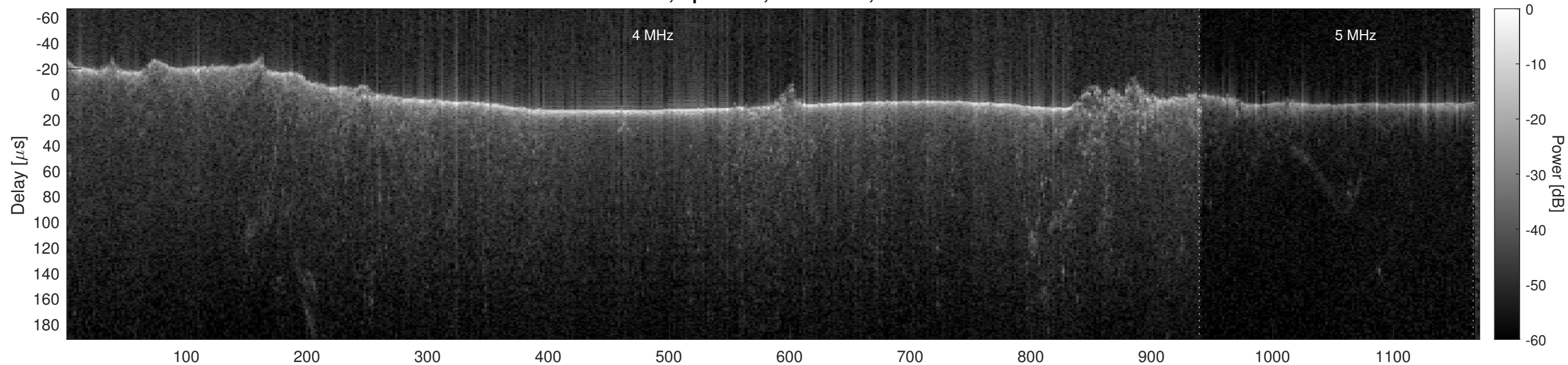
Orbit 6066, Optimized, No Window, Channel 2
