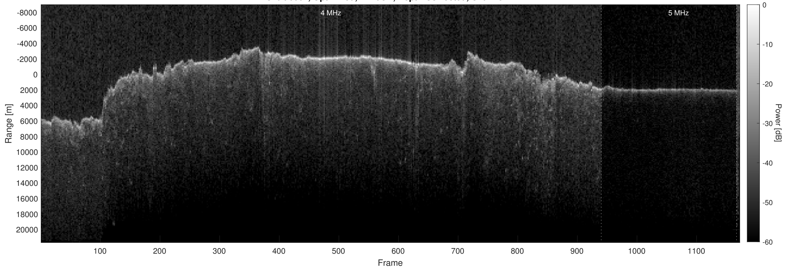
Orbit 6067, Optimized, Window, Depth-Corrected, Channel 2
