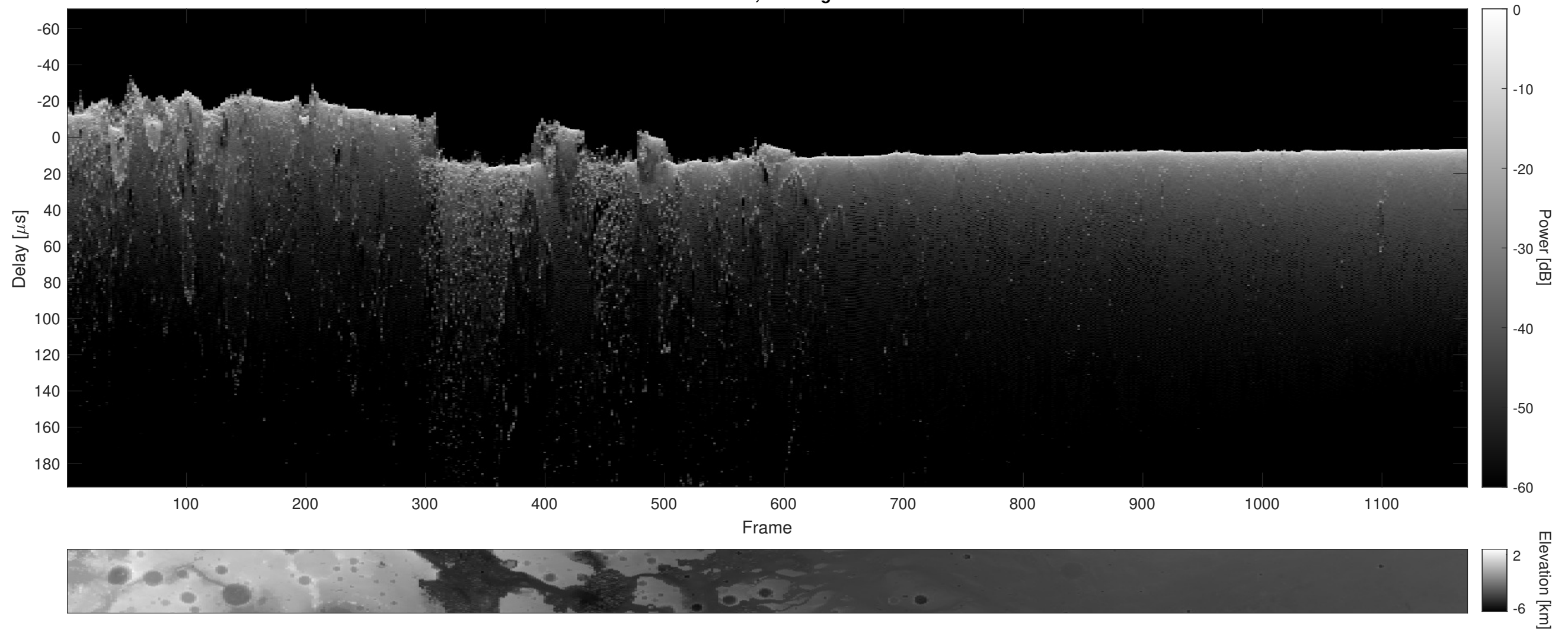
Orbit 6068, Cluttergram
