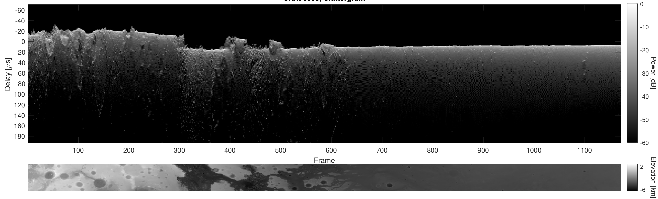
Orbit 6068, Cluttergram
