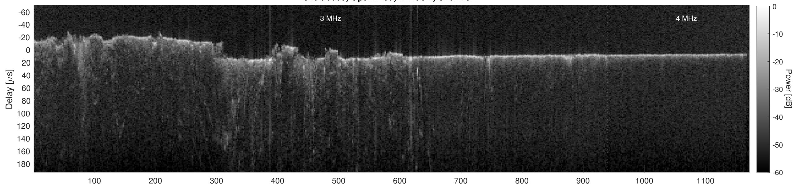
Orbit 6068, Cluttergram
