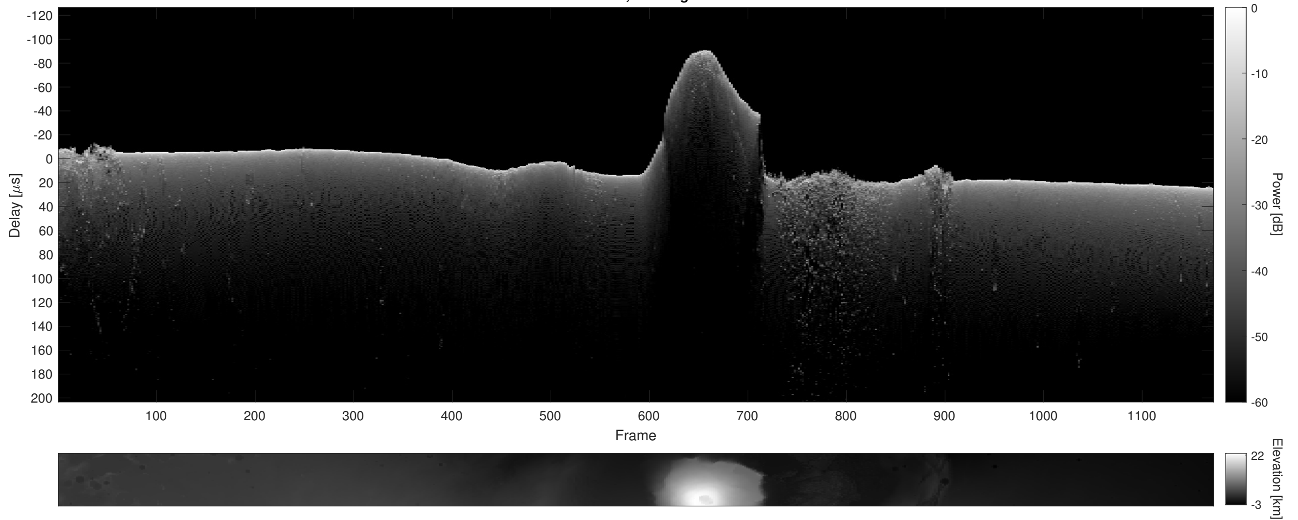
Orbit 6069, Cluttergram
