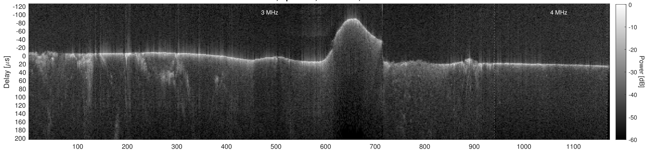
Orbit 6069, Cluttergram
