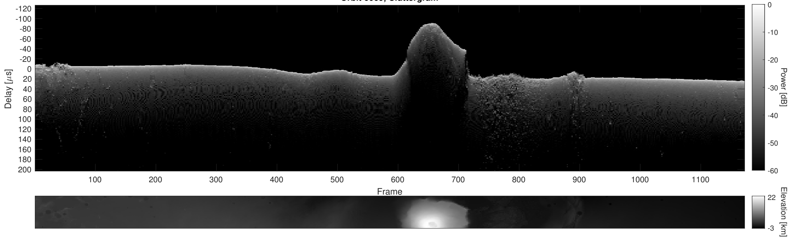
Orbit 6069, Cluttergram
