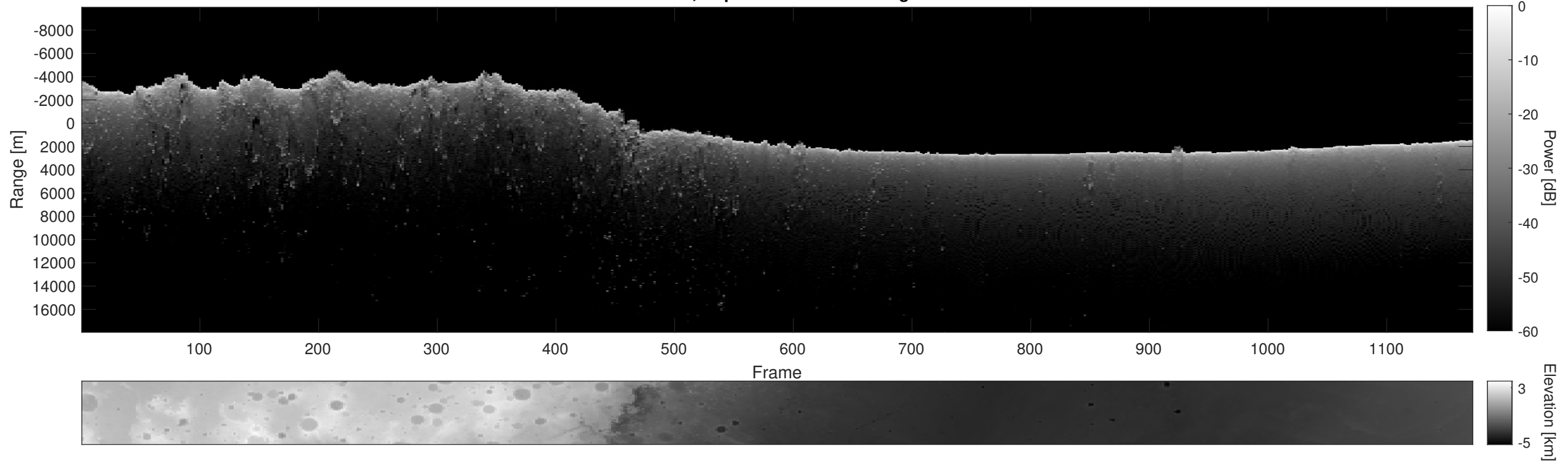
Orbit 6070, Depth-Corrected Cluttergram
