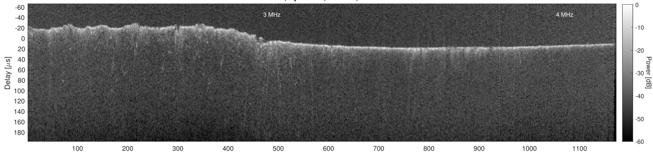
Orbit 6070, Cluttergram
